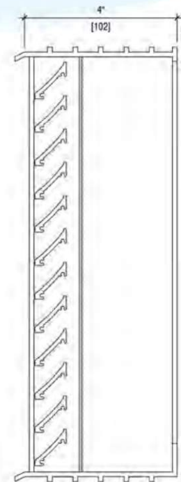
VERTICAL SECTION
